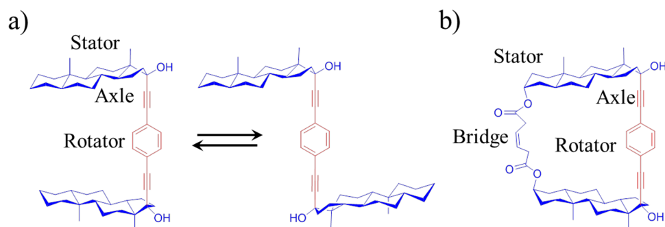
Figure 1. Line diagram of (a) conformationally unrestricted steroidal molecular rotors and (b) structure of one of the conformationally restricted molecular rotors studied in this work.
